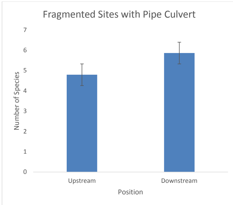
Figure 9: For sites with a physical barrier classified as a pipe culvert, species richness downstream of structure (mean = 5.86 species) vs. upstream of structure (mean = 4.79 species). Error bars give the standard error. The difference in means is statistically significant (paired t-test; p < 0.05 ).
